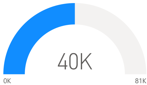
Sum of passengers
