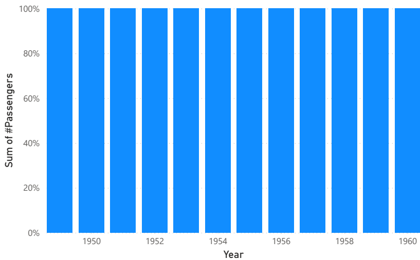
Sum of passengers
