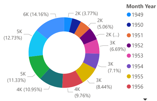
Sum of passengers
